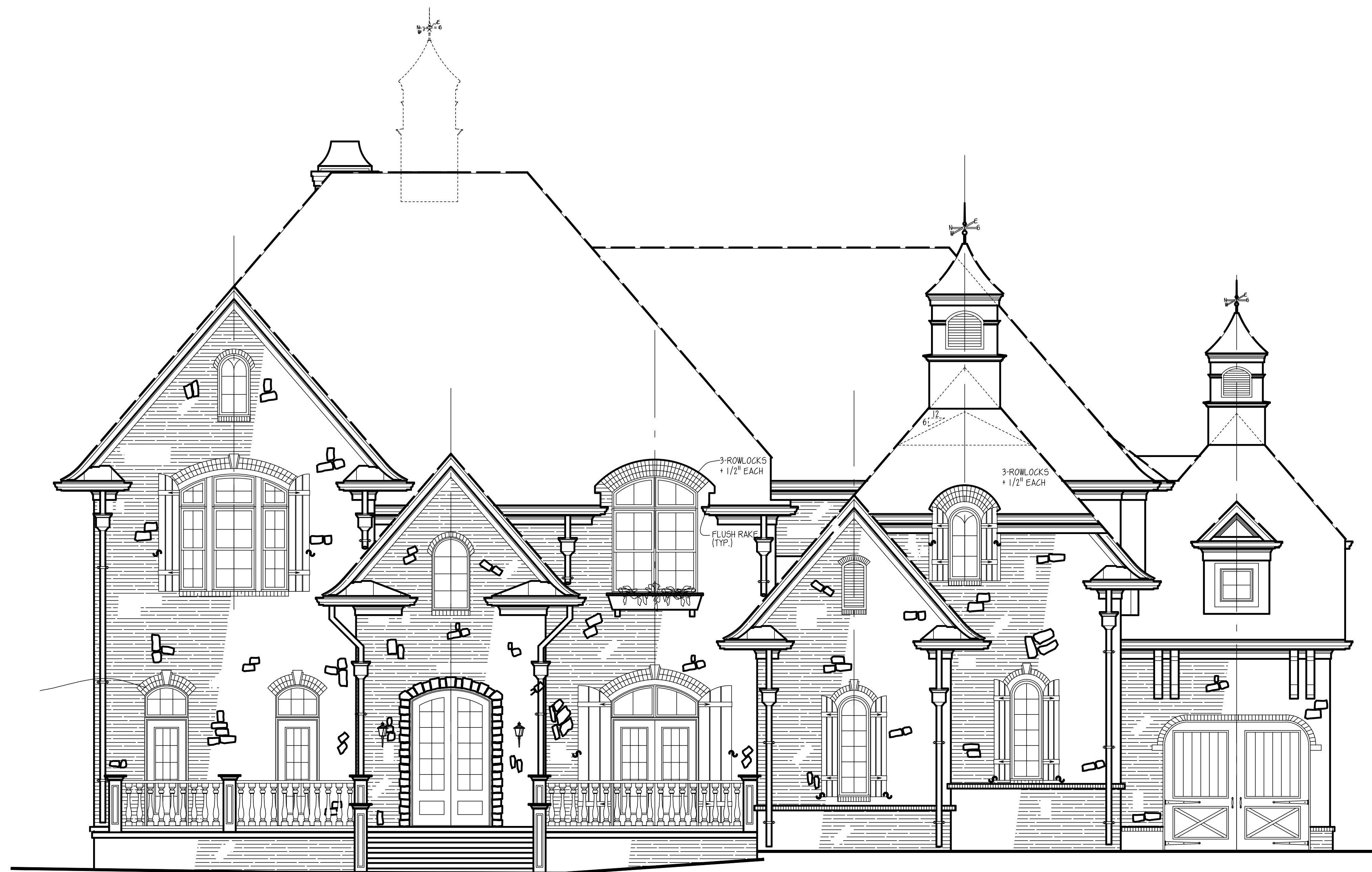
FRONT ELEVATION-"B" (SHOW HOUSE)
